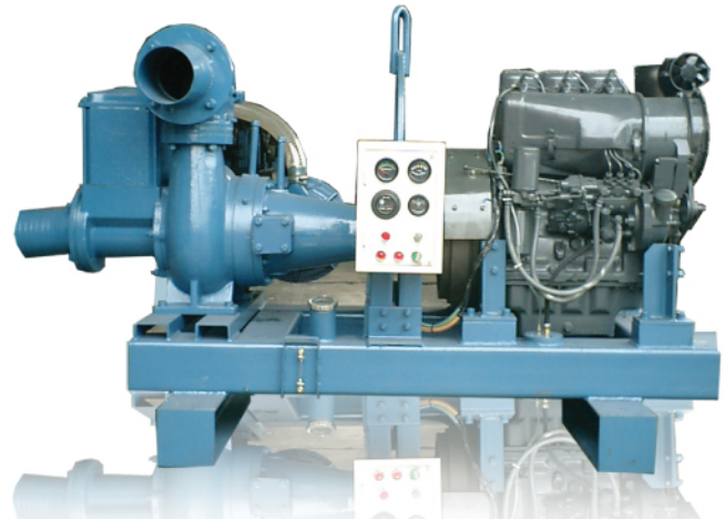
DIESEL ENGINE F3L912
